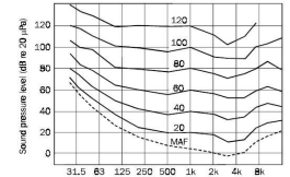
Figure 1.8. Loudness level (equal-loudness) contours, internationally standardized for pure tones heard under standard condition (ISO 226). Equal-loudness contours are determined relative to the reference level at 1000 Hz. All levels are determined in the absence of the subject, after subject level adjustment. MAF means minimum audible field.
