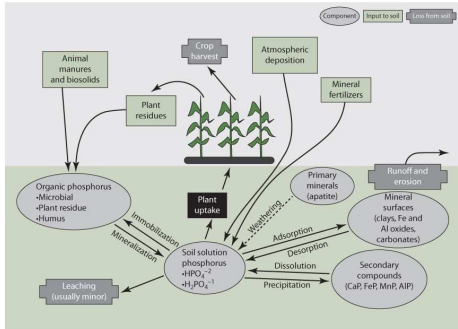
Figure 2.4 The Phosphorus Cycle
