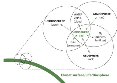
Figure 2.5 Transactions Between Atmosphere, Geosphere, and Hydrosphere Provide a Basis for the Earth's Capacity to Support Life
