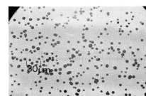
Fig. 6. Sulphuric acid mist particles deposited on AMCP 1 Stage No. 4 filter paper (X1000).
