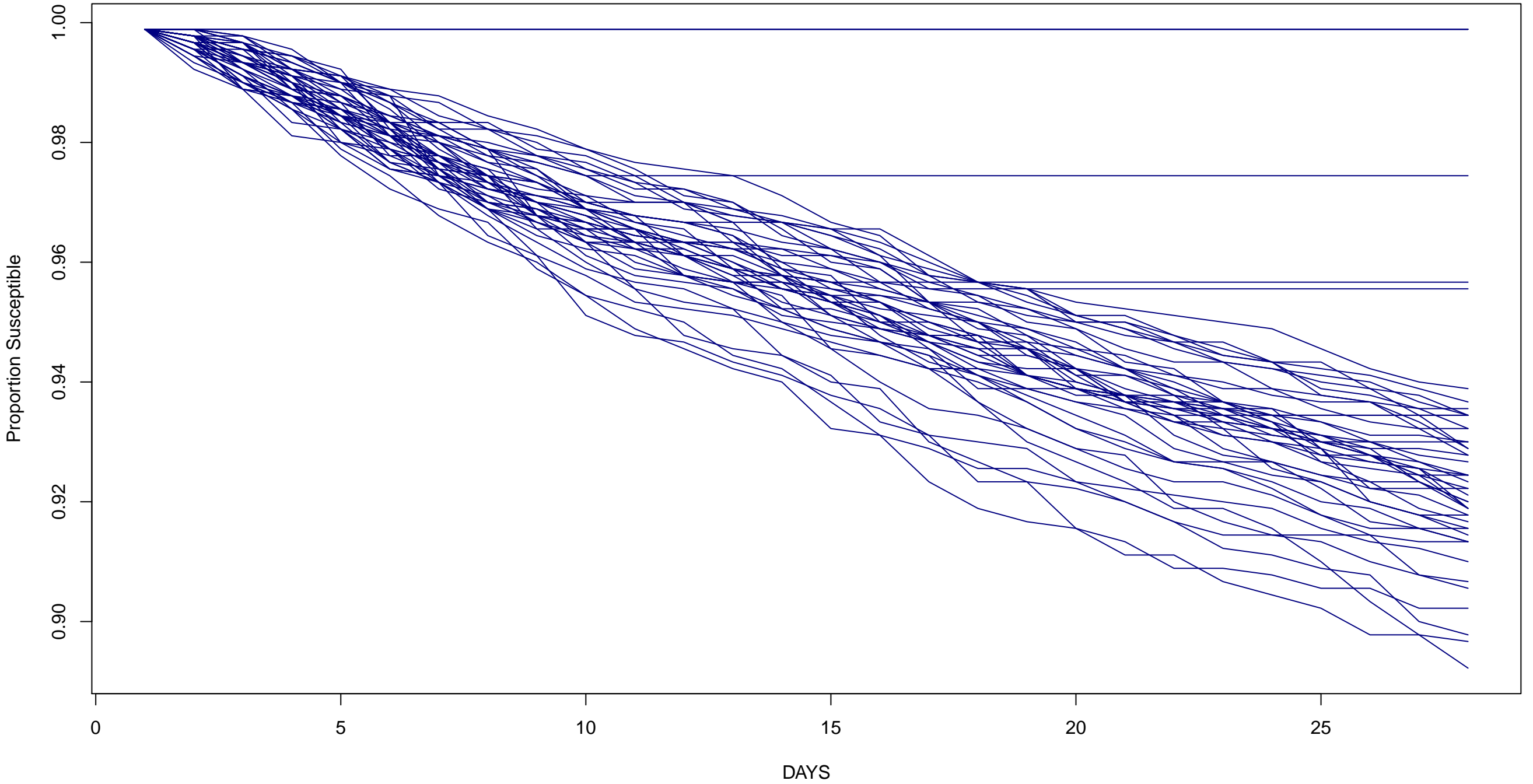
Remaining susceptibles with contacts inversely proportional to distance
