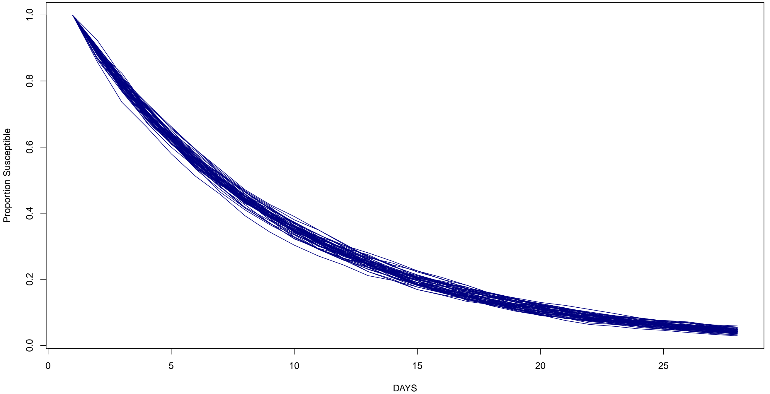
Remaining susceptible with random contacts
