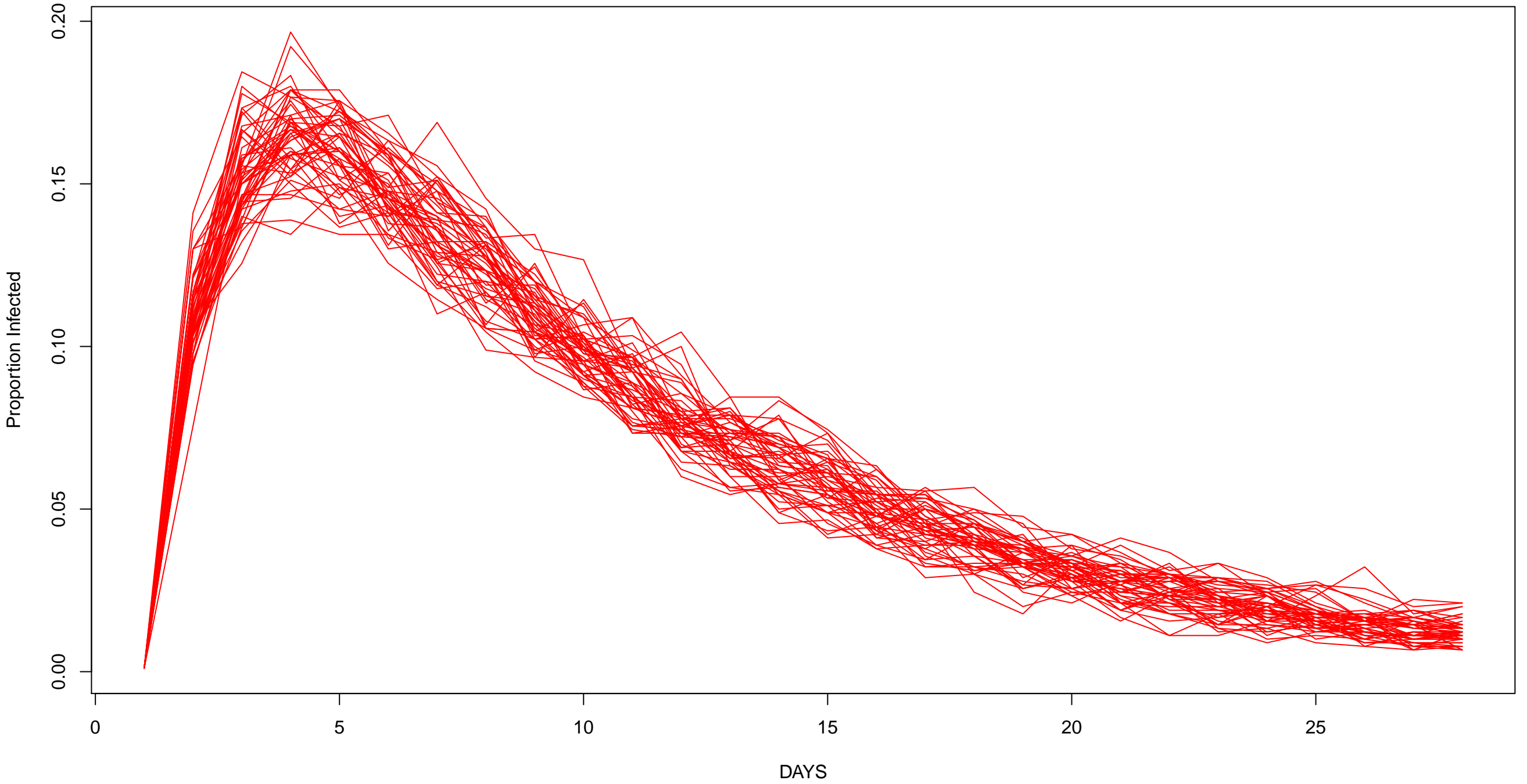
Epidemic curve with random contacts
