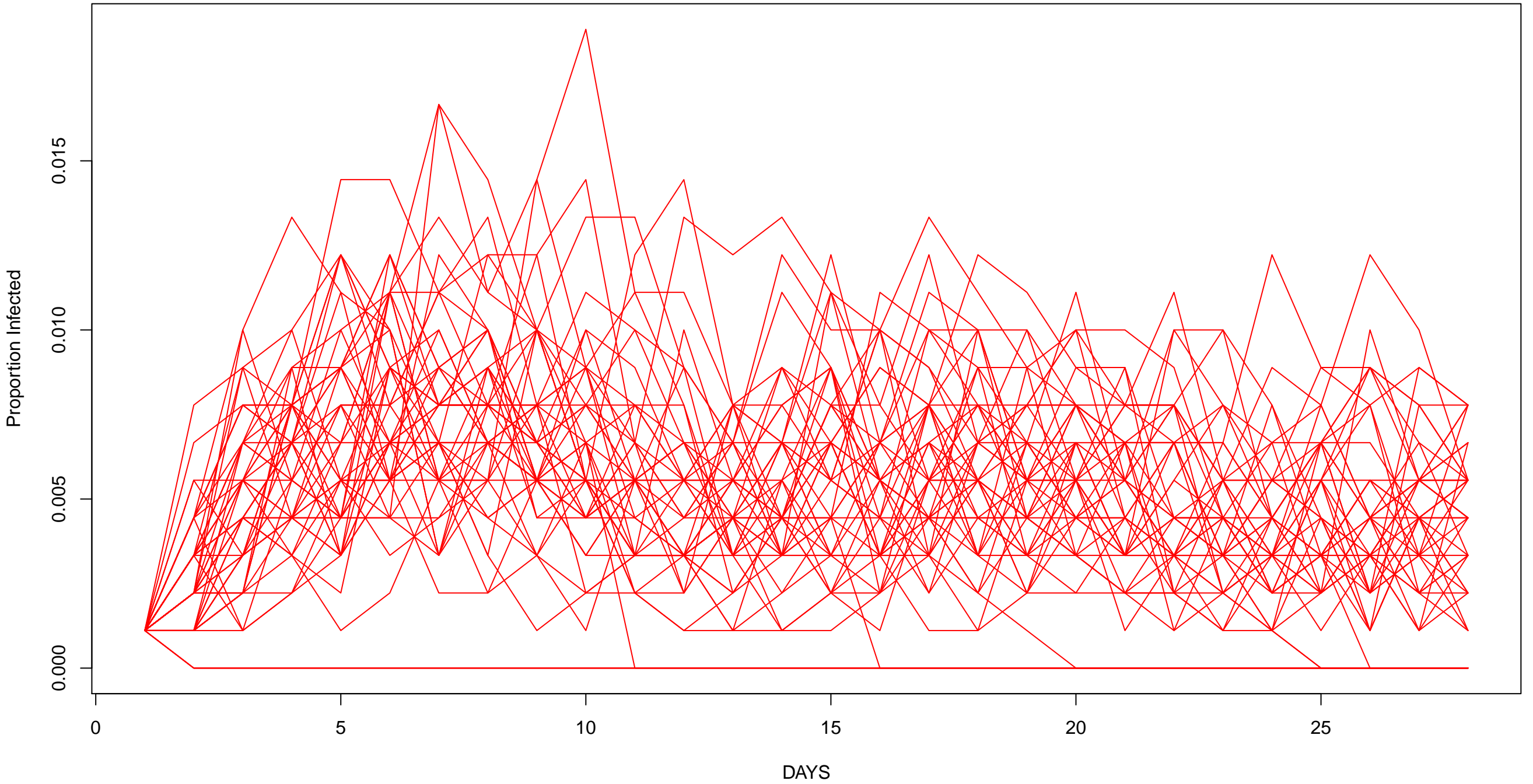
Epidemic curve with contacts inversely proportional to distance
